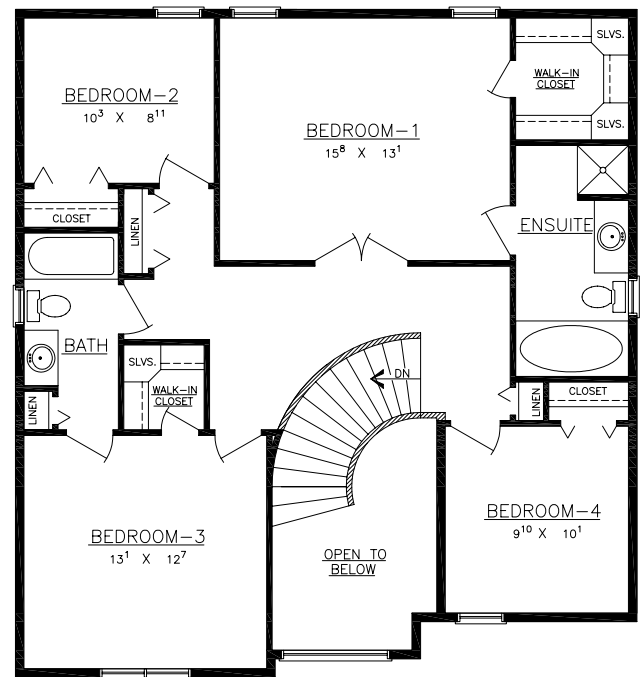
SECOND FLOOR AREA = 1026 S.F.
